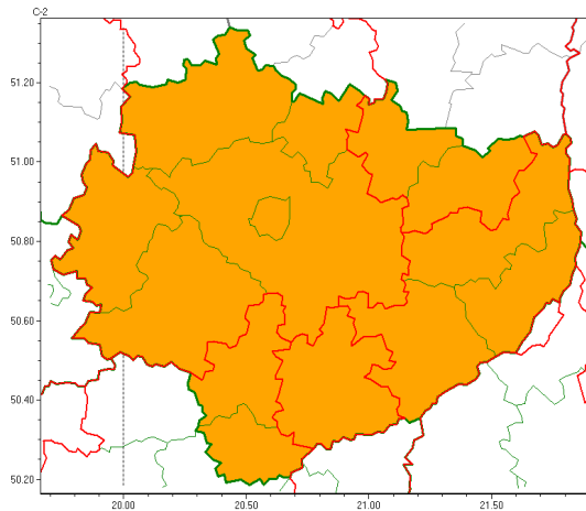
Burze z gradem 2022-06-28 14:46
